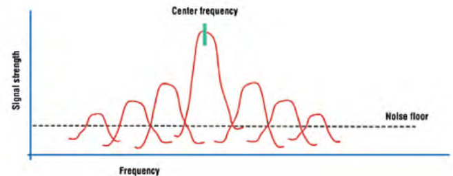
Figure 5. A Direct-sequence spread-spectrum transmission.
